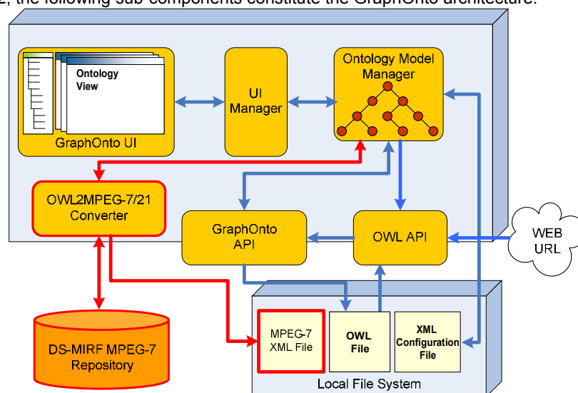
Figure 2: GraphOnto Architecture
